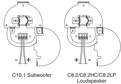
Figure 12: Subwoofer polarity with C8.2/C8.2HC/C8.2LP
